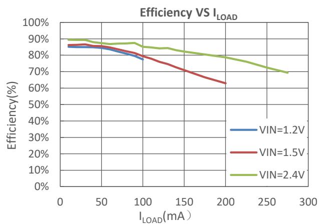
图2. Efficiency VS I_{LOAD} ( L=22\mu H )
